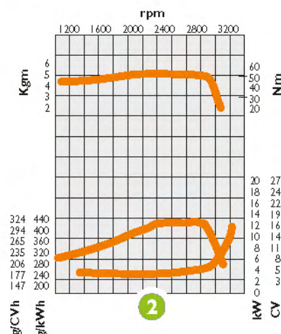
1- Performance curve 3TNV76 2- Performance curve 3TNV70
